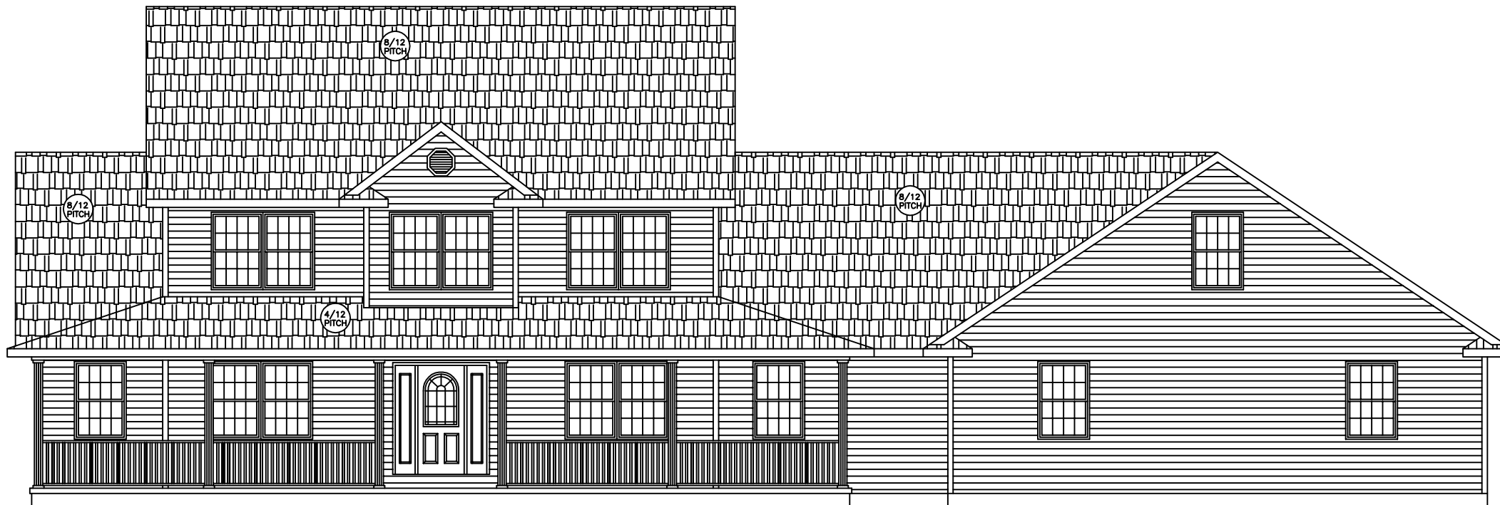
FRONT ELEVATION
